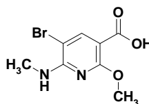
5-bromo-2-methoxy-6-(methylamino)nicotinic acid
