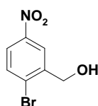
(2-bromo-5-nitrophenyl)methanol
