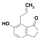
7-allyl-6-hydroxy-1-indanone
