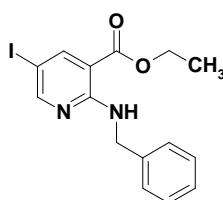
ethyl 2-(benzylamino)-5-iodonicotinate
