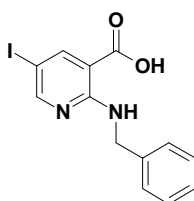
2-(benzylamino)-5-iodonicotinic acid
