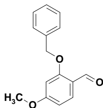
2-(benzyloxy)-4-methoxybenzaldehyde
