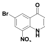
6-bromo-8-nitro-4(1H)-quinolinone
