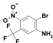
2-bromo-4-nitro-5-(trifluoromethyl)aniline
